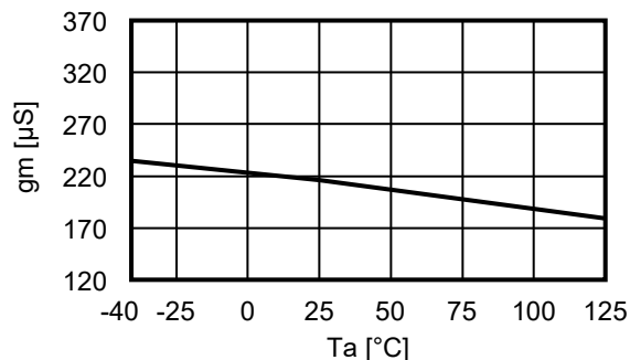
2. 13 Error amplifier transconductance ( g_m ) vs. Temperature ( T_a )
