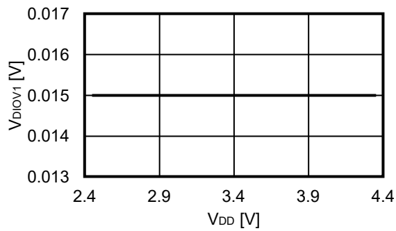
2.5 V_{DIOV1} - V_{DD}
