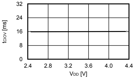
3.9 t_{CI0V} - V_{DD}
