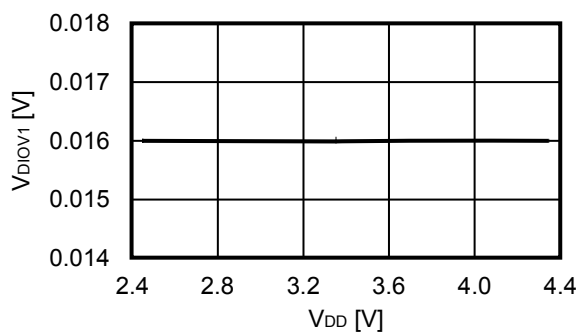
2.5 V_{DIOV1} - V_{DD}
