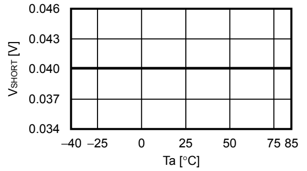
2.10 V_{SHORT} - T_a
