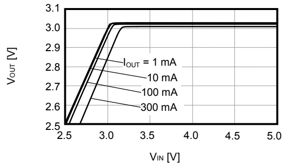
S-1170B30 (Ta=25°C)
