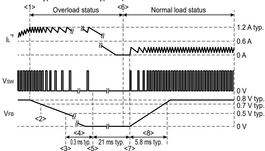
*1. Inductor current
