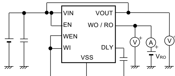
Figure 16 Test Circuit 6
