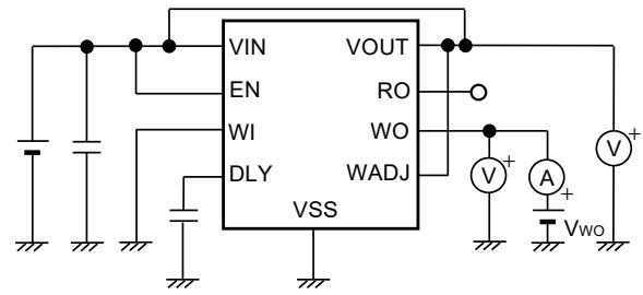
Figure 32 Test Circuit 12
