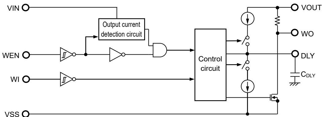
Figure 40 Operation of Watchdog Timer Block
