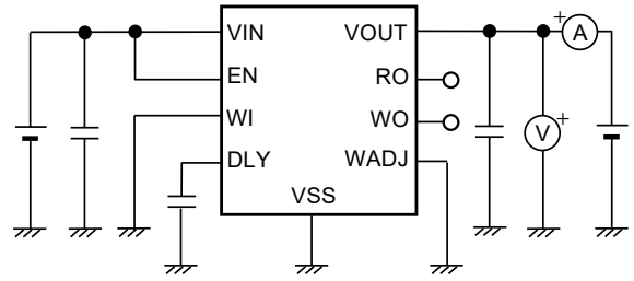
Figure 22 Test Circuit 2
