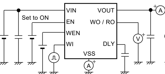
Figure 19 Test Circuit 9
