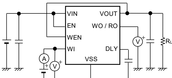
Figure 17 Test Circuit 7
