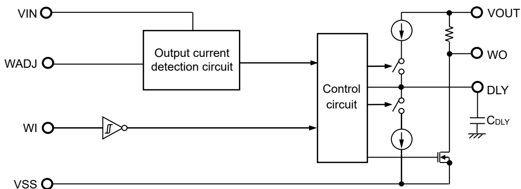
Figure 44 Operation of Watchdog Timer Block
