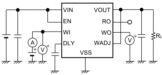
Figure 31 Test Circuit 11
