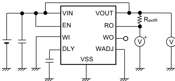
Figure 25 Test Circuit 5
