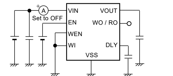
Figure 20 Test Circuit 10
