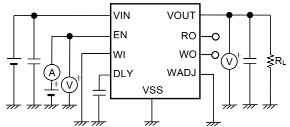
Figure 24 Test Circuit 4
