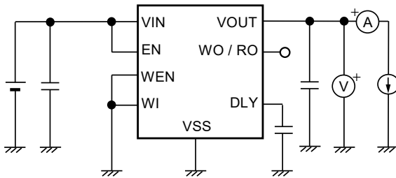
Figure 11 Test Circuit 1
