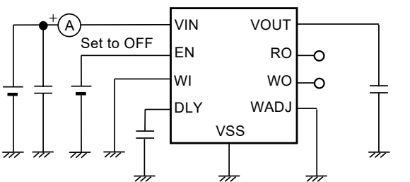
Figure 30 Test Circuit 10
