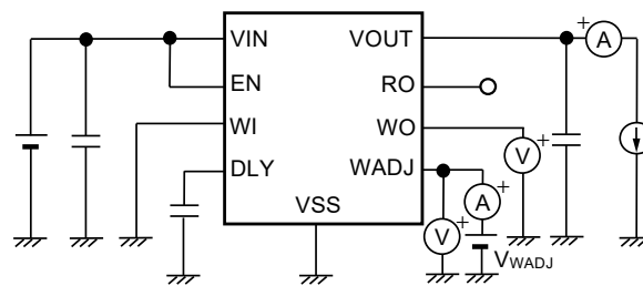
Figure 28 Test Circuit 8
