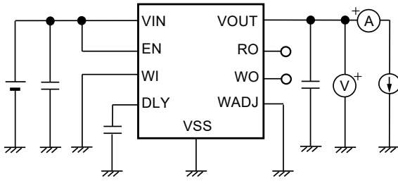
Figure 21 Test Circuit 1
