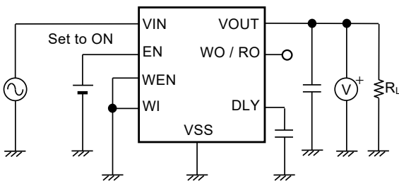
Figure 13 Test Circuit 3
