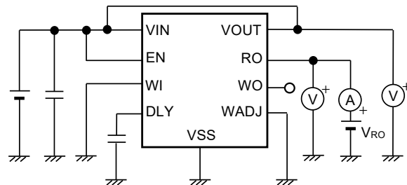
Figure 26 Test Circuit 6
