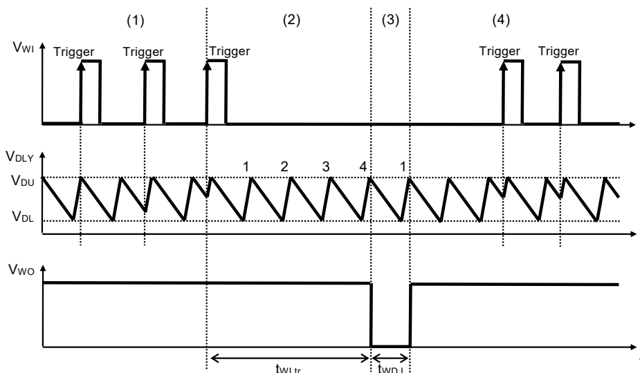
Figure 39 Timing Chart of Watchdog Timer Block
