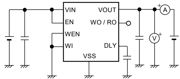
Figure 12 Test Circuit 2
