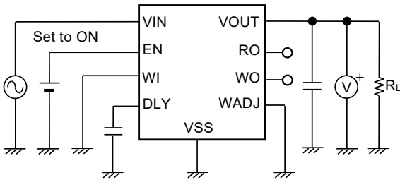
Figure 23 Test Circuit 3
