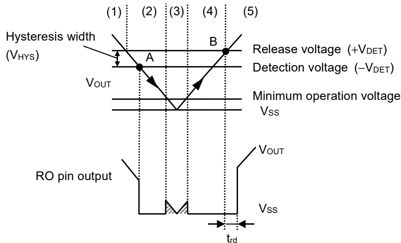
Figure 38 Timing Chart of Detector Block
