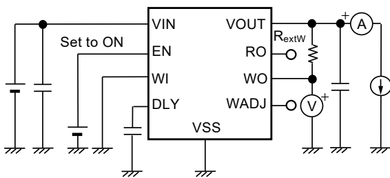
Figure 27 Test Circuit 7
