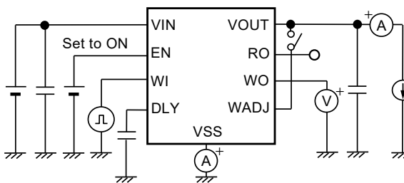
Figure 29 Test Circuit 9
