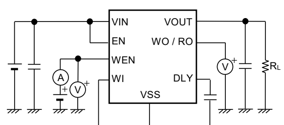
Figure 18 Test Circuit 8
