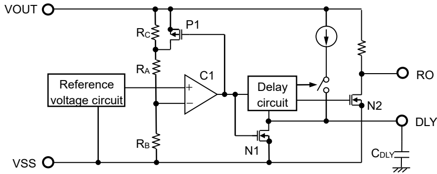
Figure 37 Operation of Detector Block
