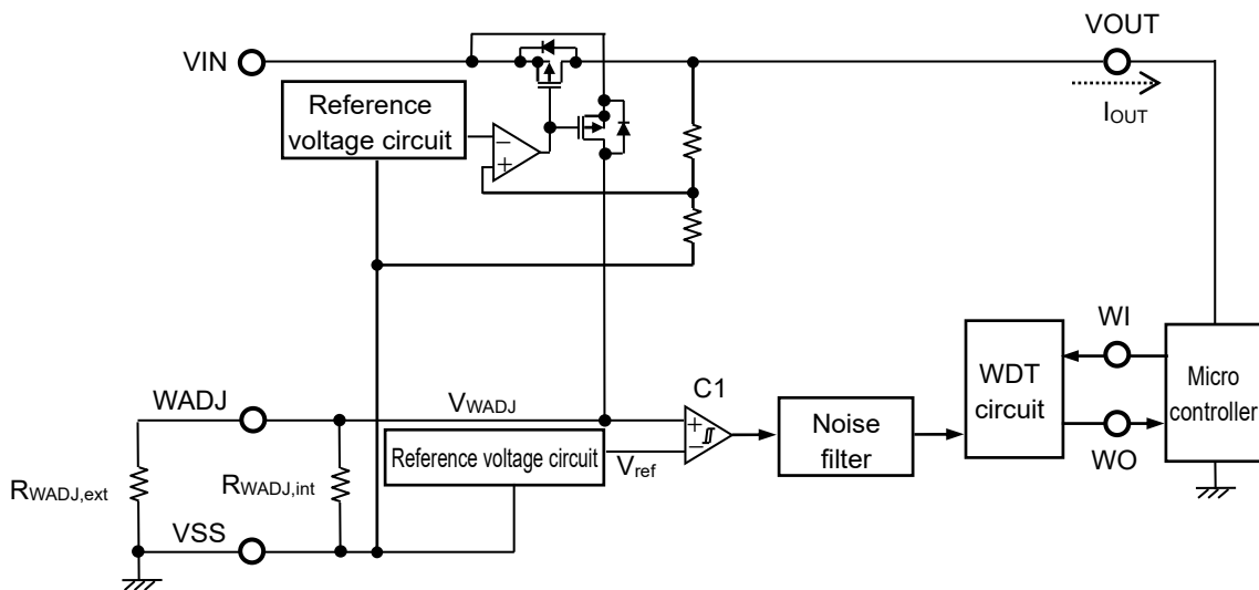
Figure 45 Operation of Output current Detection Circuit
