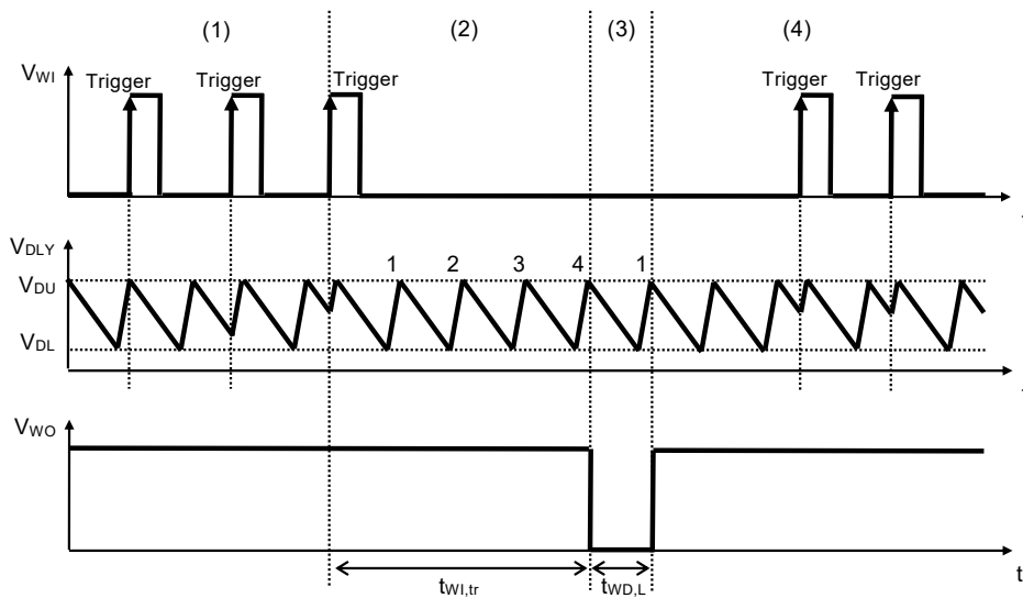
Figure 43 Timing Chart of Watchdog Timer Block
