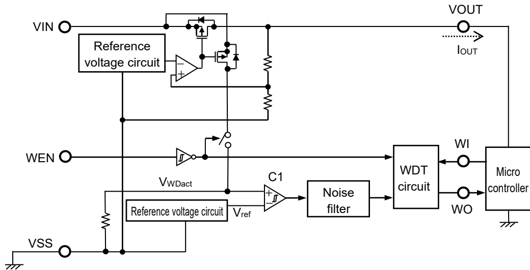
Figure 41 Operation of Output Current Detection Circuit
