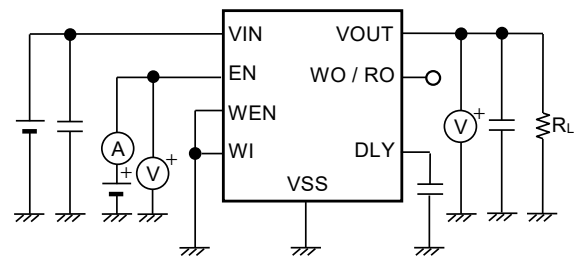
Figure 14 Test Circuit 4
