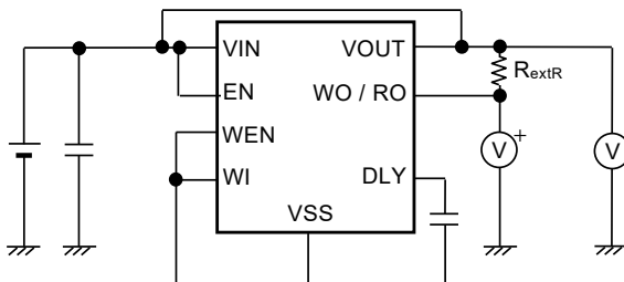
Figure 15 Test Circuit 5
