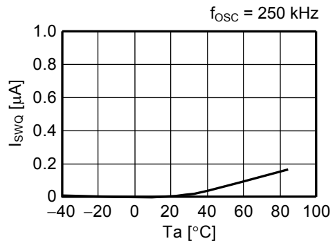
(5) Switching Transistor Leakage Current ( I_{\text{SWQ}} ) vs. Temperature ( T_a )
