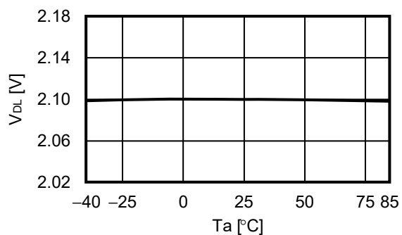
2.3 V_{DL} - T_a
