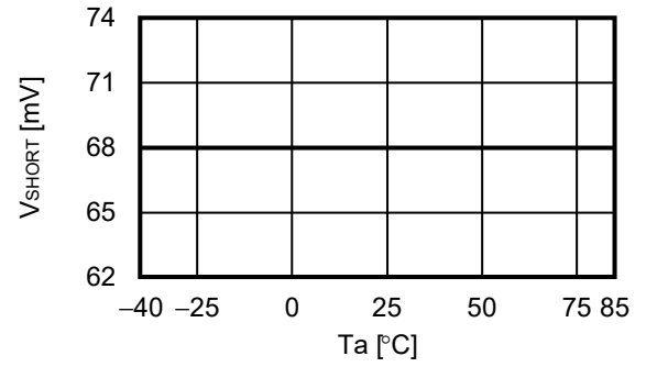
2.10 V_{SHORT} - Ta
