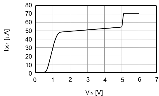
S-1170B50 ( T_a=25^\circ\text{C} )
